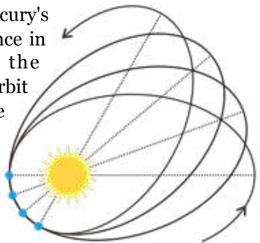
The precession of the perihelion of Mercury causes its orbit to rotate slowly and hence the planet no longer follows closed orbits.
