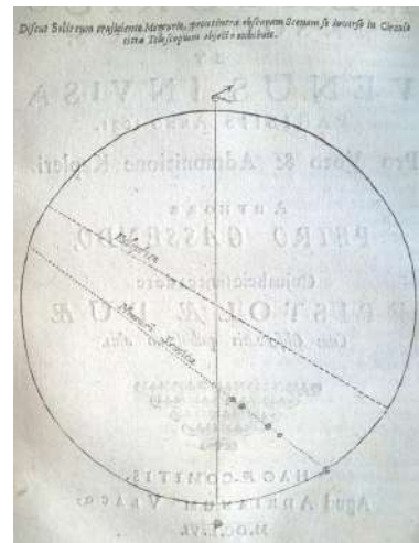
Gassendi's drawing of the transit of Mercury in 1631. Image credit: RAS
