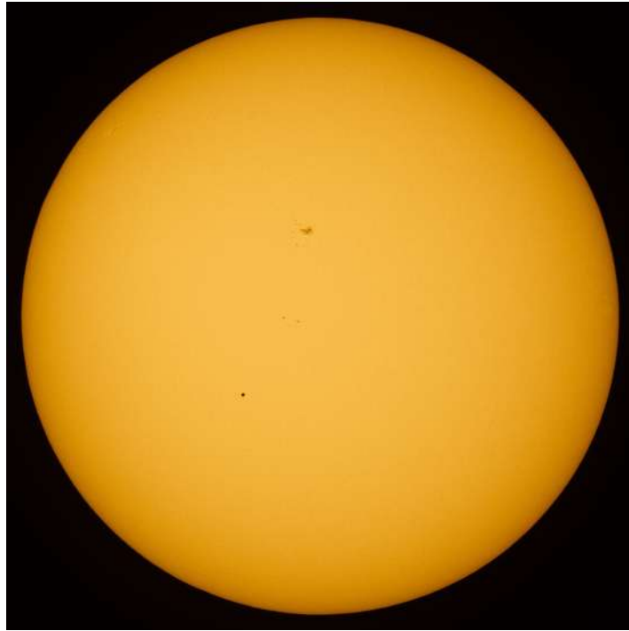
Transit of Mercury, 9 May 2016, photographed by Elijah Mathews. The sharp dot left and below the centre is Mercury and the fuzzy spot higher up is a sunspot
